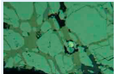
Classic example of gold (electrum Ag, Au) entrapment in a particle comprising chalcopyrite cemented pyrite micro-breccia. The larger gold granule is 5x6mm.
